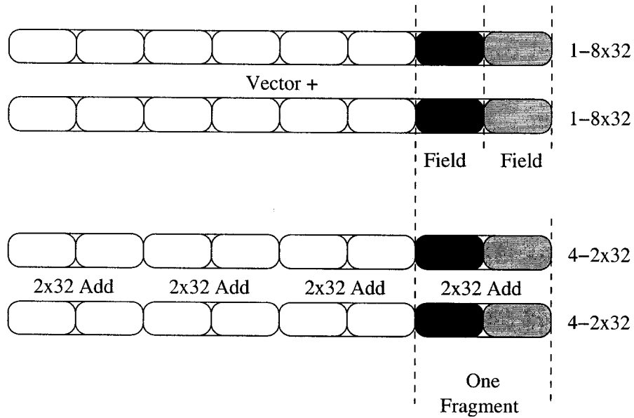
Fig. 4.2. Fragmentation of a Vector Addition
