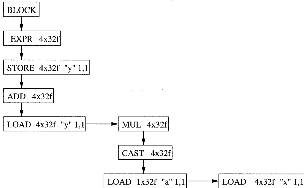
Fig. 4.1. IR tree for SWAR SAXPY
